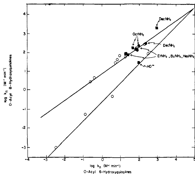
Figure 4. Plot of \log k_n for the reaction of nucleophiles with E8-Ac vs. \log k_n for reaction of the same nucleophiles with E6-Ac. The open circles represent data for various nucleophiles taken from ref 3. The solid squares are values obtained in this study for octanoates; the solid circles are values for the acetates.
