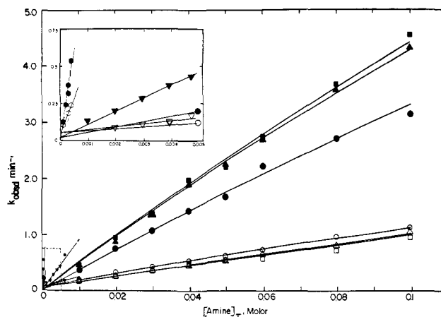
Figure 3. Plots of k_{\text{obsd}} vs. [amine] T for the reaction of E6-Oct (open symbols) and E8-Oct (solid symbols) with ethyl- ( \circ ), butyl- ( \Delta ), hexyl- ( \square ), octyl- ( \nabla ), and decylamines ( \circ ). The insert is a partial enlargement of the region enclosed by the dashed line. All solutions were at pH 10.60.
