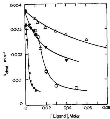
Figure 2. Plots of k_{\text{obsd}} vs. [ligand] for the hydrolysis of E8-Ac in the presence of A-10 + ( \Delta ) and DPB ( \blacktriangledown ) and for the hydrolysis of E8-Hex in the presence of A-10 + ( \circ ) and DPB ( \blacksquare ). All solutions were at pH 4.6 in 0.4 M acetate buffer.
