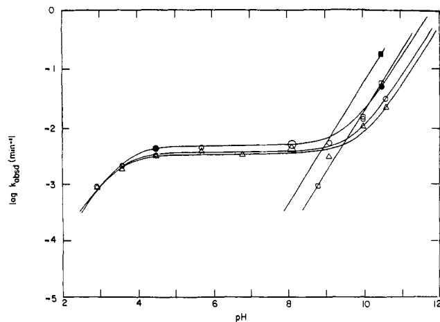
Figure 1. pH-log k_{obsd} profiles for the hydrolysis of esters E8-Ac (●), E6-Ac (■), E8-Hex (○), E8-Oct (△), and E6-Oct (□). The plots for E8-Ac and E6-Ac are derived from the data of ref 3.
